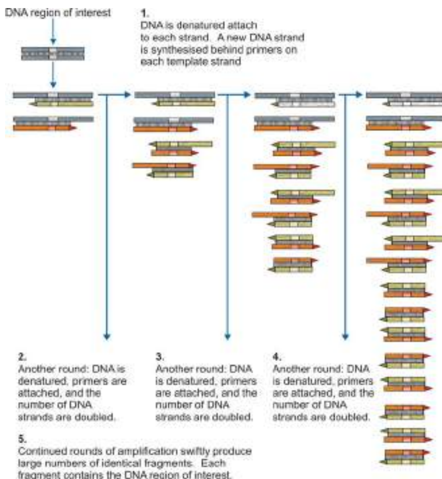
Fig. 12.5: A schematic diagram showing the process of polymerase chain reaction. Orange and green arrows show the forward and reverse primers respectively ( Courtesy: Human genome database )
