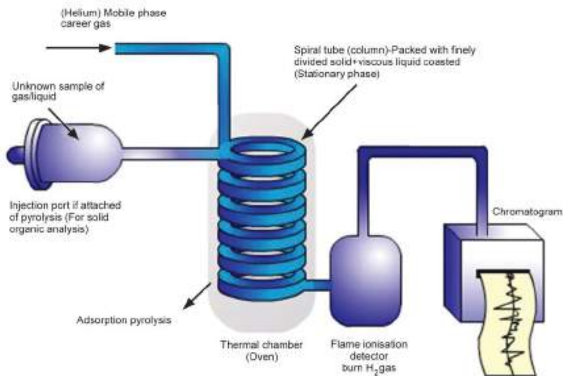
Fig. 31.5: Gas chromatography
